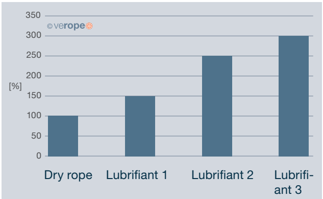
Fig. 21: Influence of the lubricant on the service life of the wire rope
