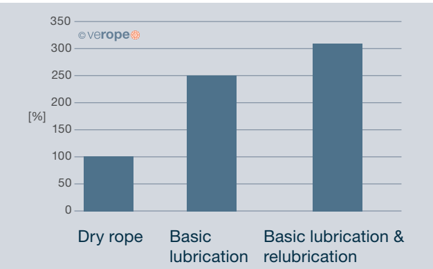
Fig. 22: Influence of relubrication on wire rope service life
