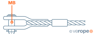
Ferrule-secured open thimble termination
