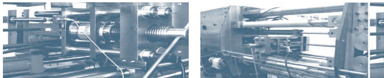
Figure 62: Testing principle of the measurement of the modulus of elasticity under load (source: TU Clausthal)
