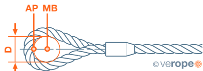
Flemish eye ferrule-secured termination
