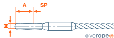
Threaded socket swaged
