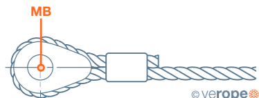
Ferrule-secured solid thimble termination
