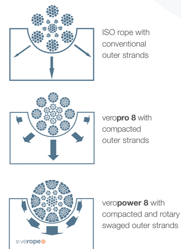
Figure 24a: Comparison wear resistance
