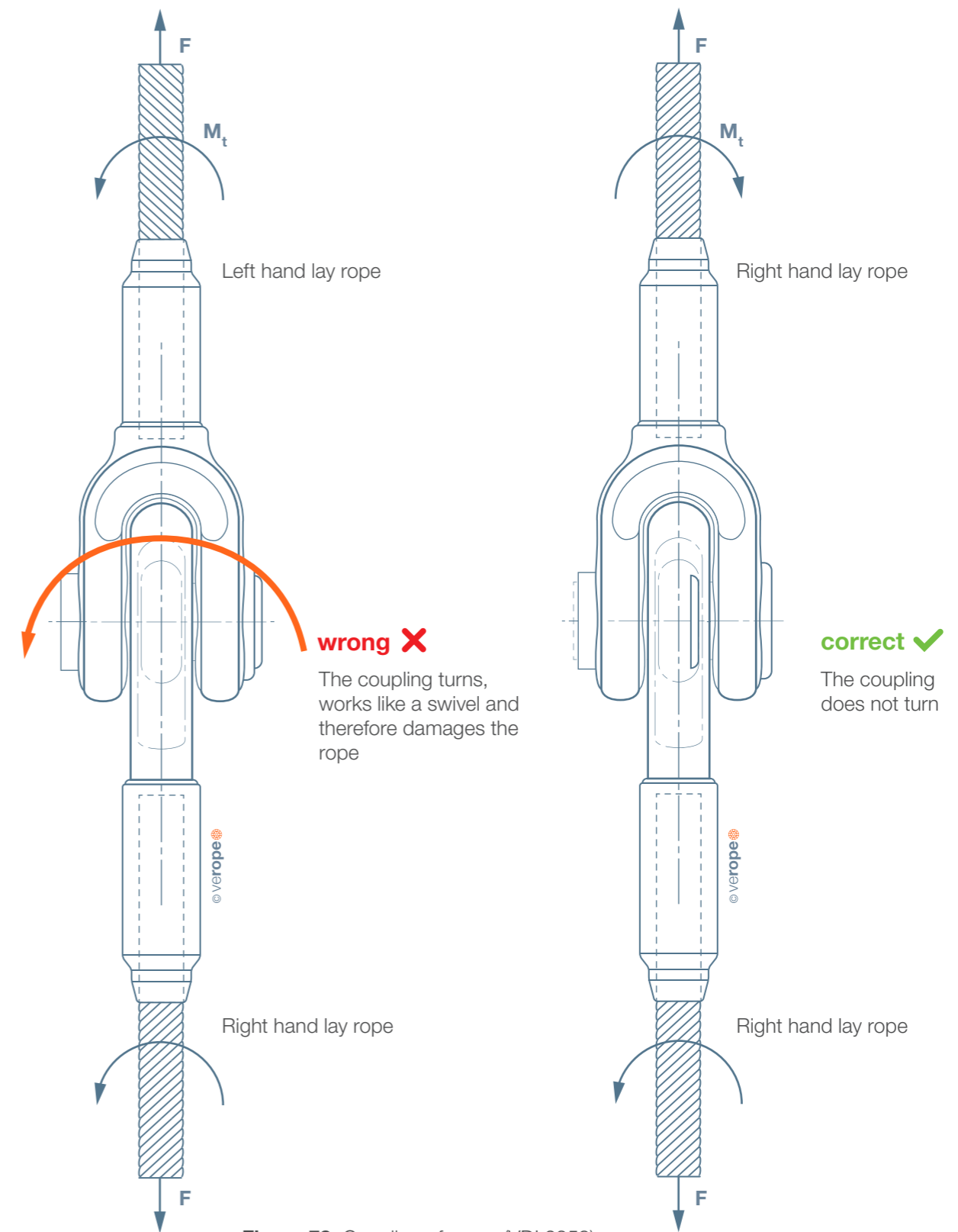
Figure 78: Coupling of ropes (VDI 2358)
