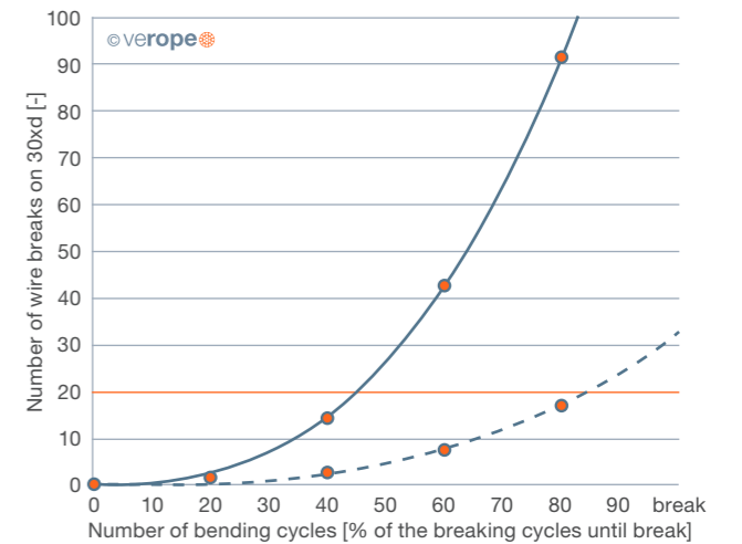
Figure 42: Number of visible (pulled trough line) and invisible wire breaks (sketched line) dependent on the rope lifetime. After the end of the bending fatigue test, the analysis of the rope sections with the different fatigue numbers show the marked numbers of wire breaks.
