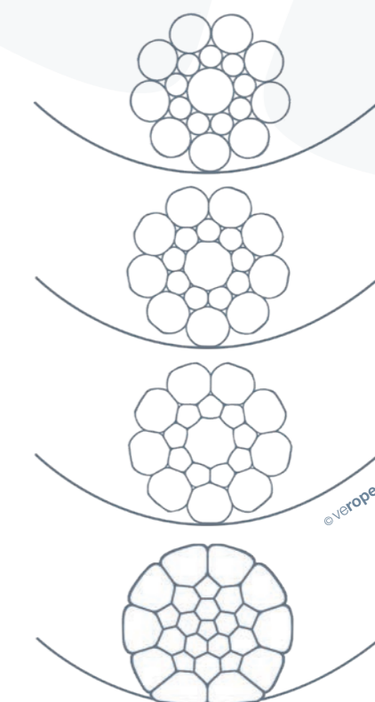
Figure 24b: Contact area of strands
