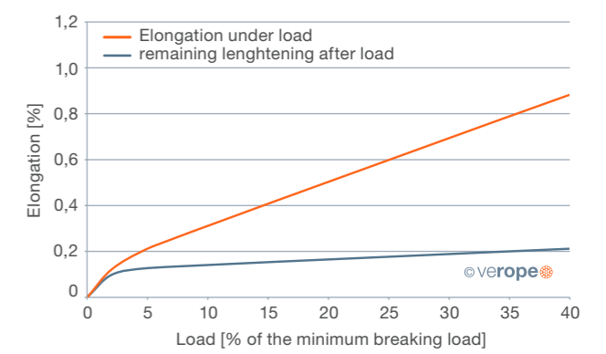
Figure 57: Elongation under load (upper graph) and remaining lengthening after load (lower graph) depending on the line pull (verotop P, regular lay, 1960 N/mm 2 )
