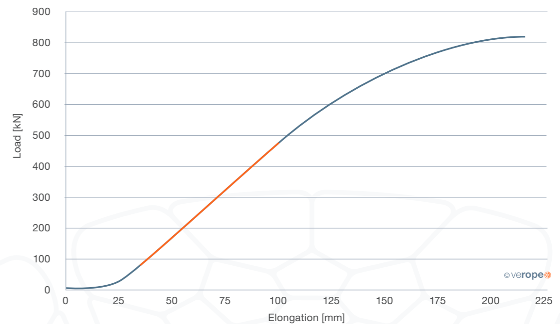
Figure 27: Load-elongation diagram of a rope
