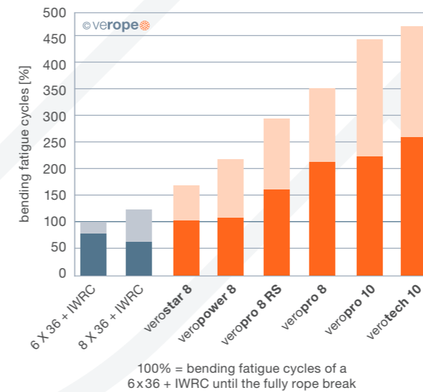
Figure 47: Number of bending cycles until discard and until break (non-rotation resistant ropes, equal load)
