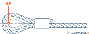
Ferrule-secured eye termination
