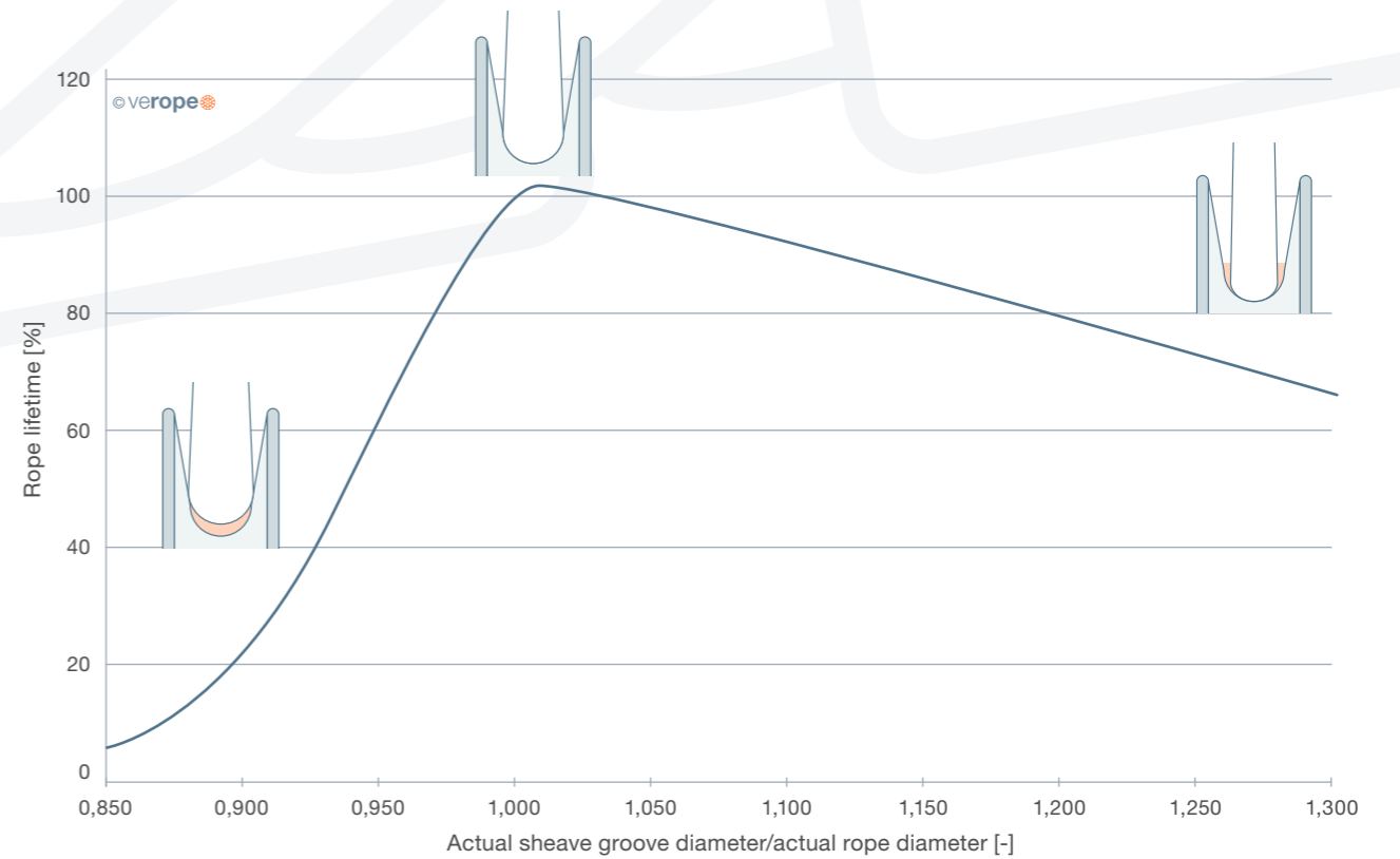
Figure 51: Influence of the groove diameter onto the rope lifetime (see also page 60)
