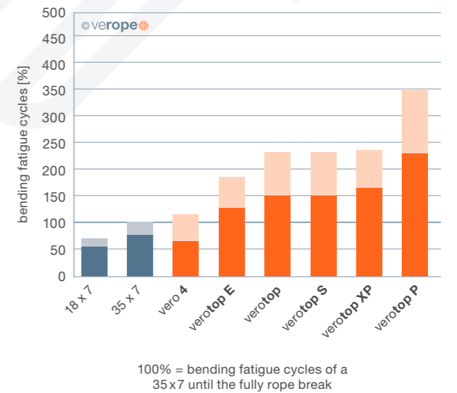
Figure 48: Number of bending cycles until discard and until break (rotation-resistant ropes, equal load)
