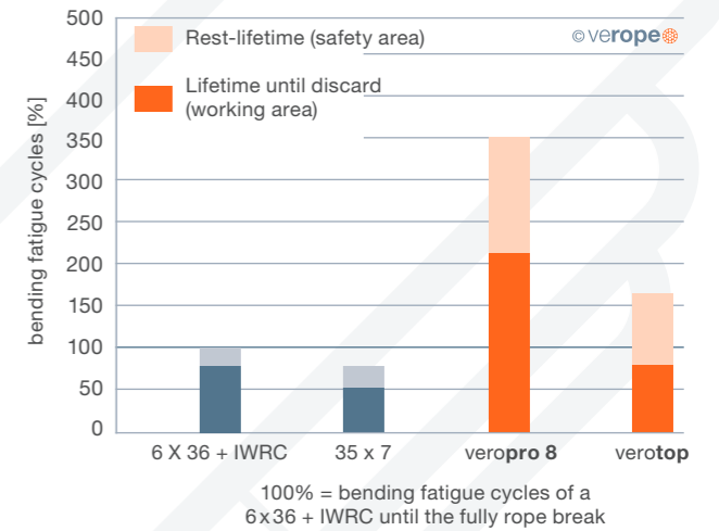
Figure 46: Number of bending cycles until discard and until break
