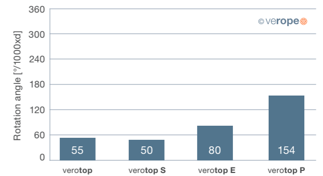
Figure 66: Rotation angle under load of 20% of the minimum breaking load
