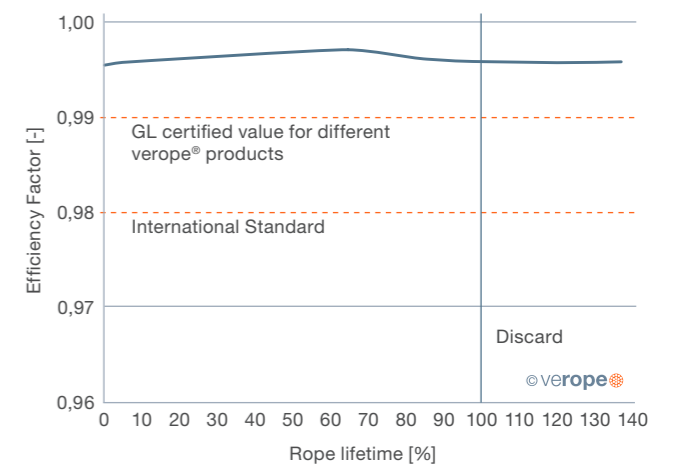
Figure 71: Efficiency factor measurement over the rope lifetime under load
