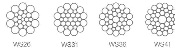
Figure 7: Strand designs
