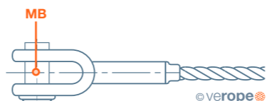
Open socket swaged
