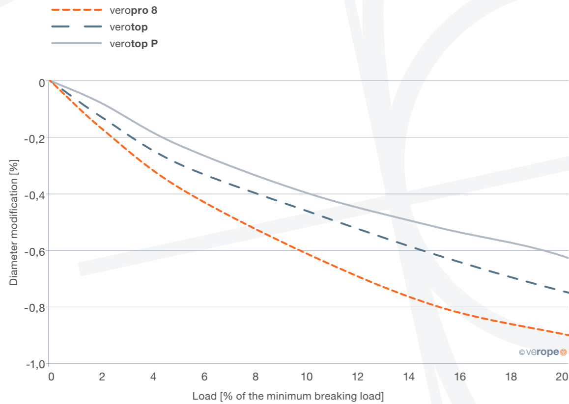
Figure 59: Diameter modification depending on the line pull
