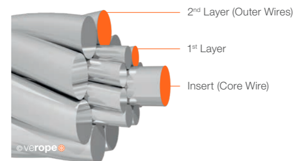
Figure 1: Components of a strand
