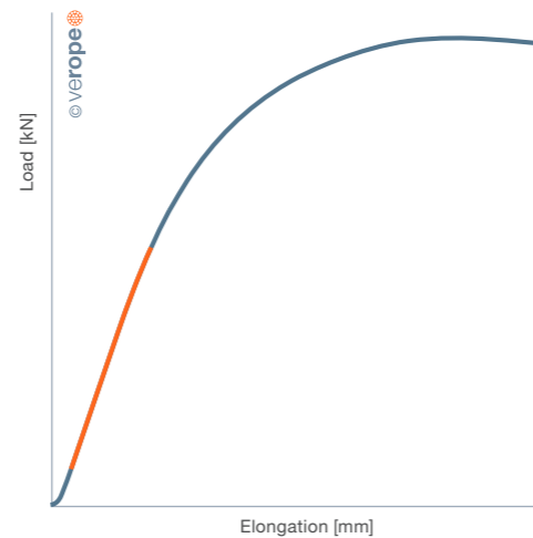
Figure 26: Load-elongation diagram of a strand
