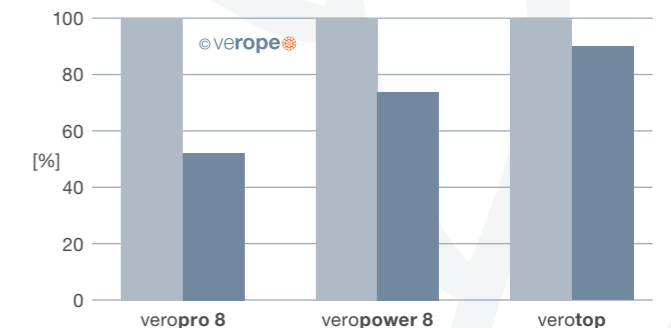
Figure 32: Breaking strengths of a rope without and with using a swivel
