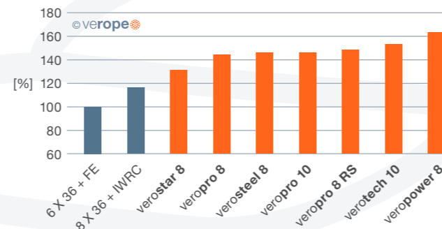
Figure 30: Breaking strengths of non-rotation resistant ropes
