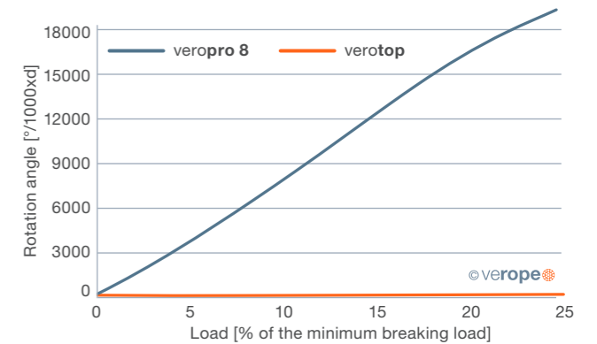
Figure 64: Rotation angle test veropro 8 and verotop
