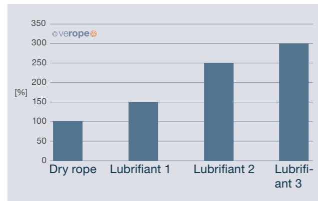
Fig. 21: Influence of the lubricant on the service life of the wire rope
