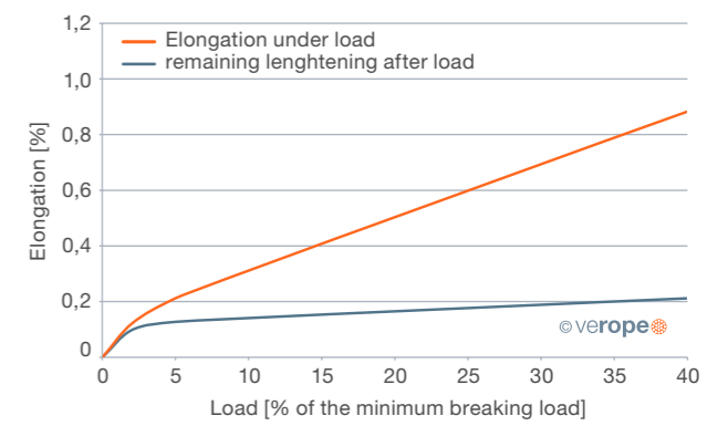
Figure 57: Elongation under load (upper graph) and remaining lengthening after load (lower graph) depending on the line pull (verotop P, regular lay, 1960 N/mm²)
