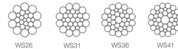
Figure 7: Strand designs
