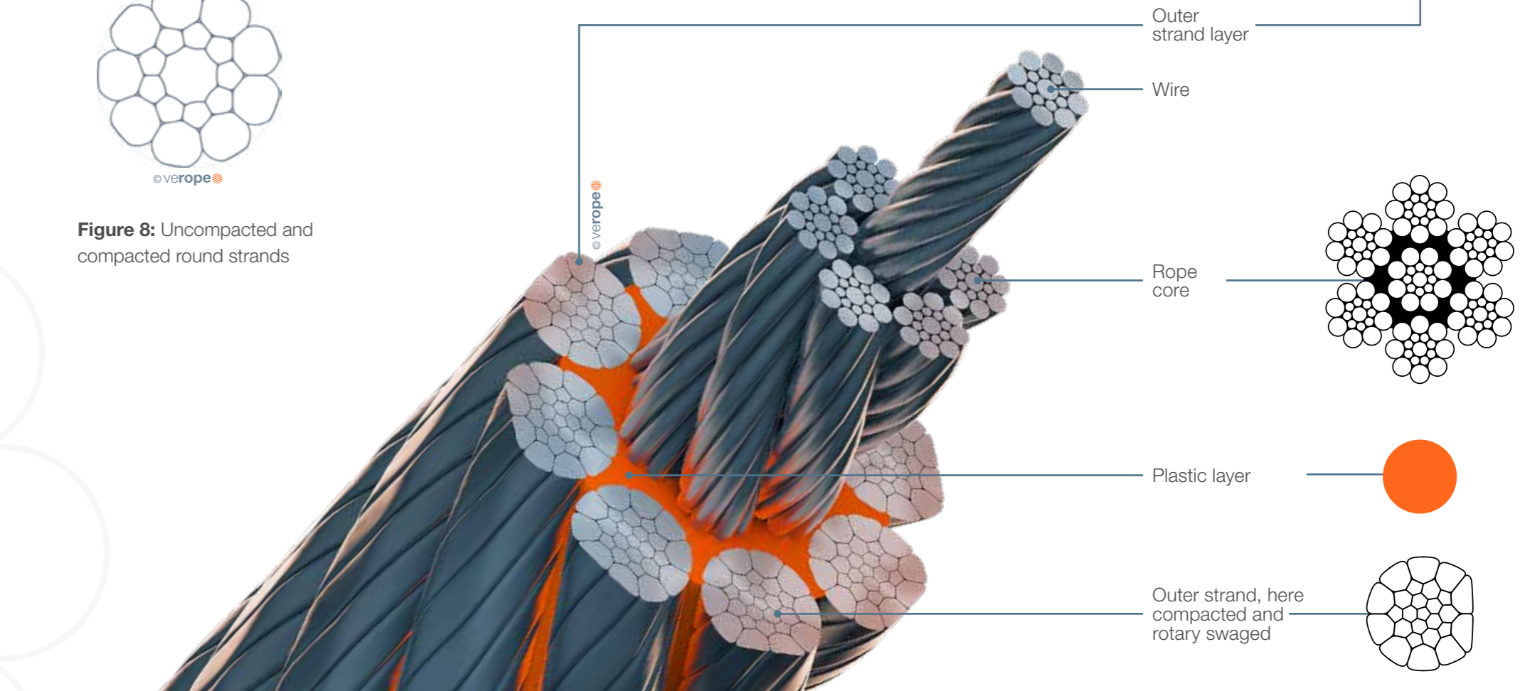
Figure 9: Composition of a special wire rope (veropro 8 RS)
