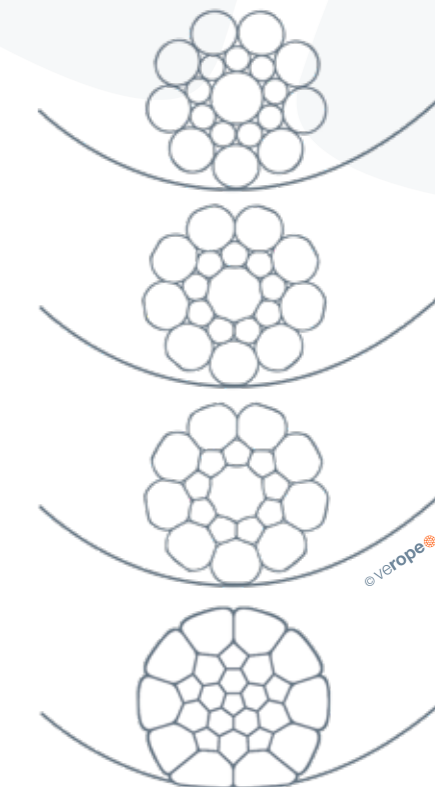
Figure 24b: Contact area of strands
