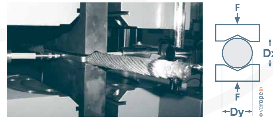
Figure 61: Testing device (source: TU Dresden)
