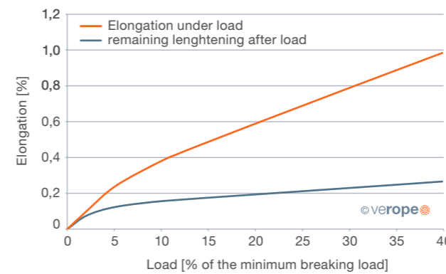
Figure 56: Elongation under load (upper graph) and remaining lengthening after load (lower graph) depending on the line pull (veropro 8, ordinary lay, 1960 N/mm²)
