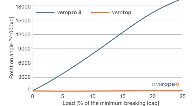
Figure 64: Rotation angle test veropro 8 and verotop
