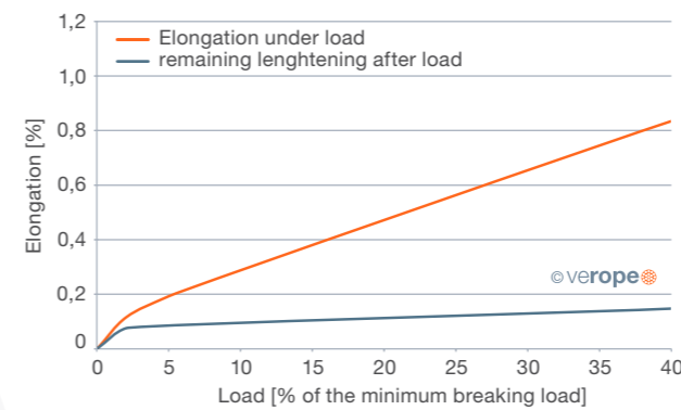
Figure 58: Elongation under load (upper graph) and remaining lengthening after load (lower graph) depending on the line pull (verotop, regular lay, 1960 N/mm²)
