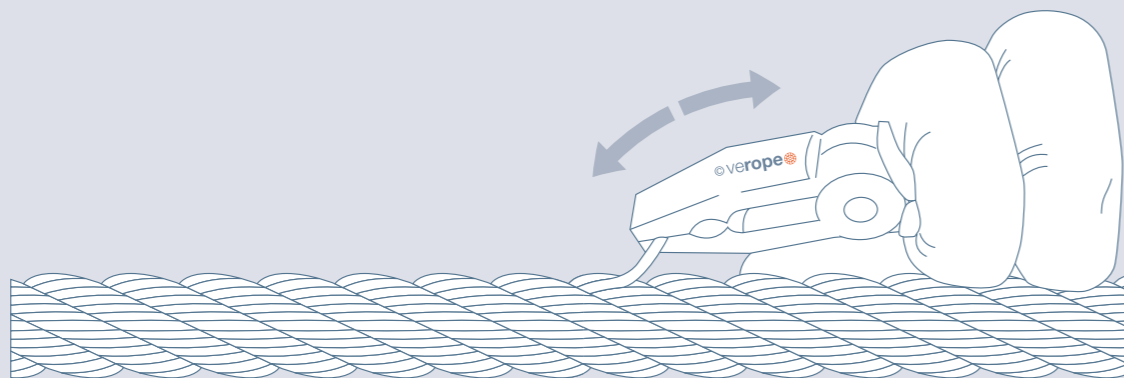
Fig. 50: Removal of wires
